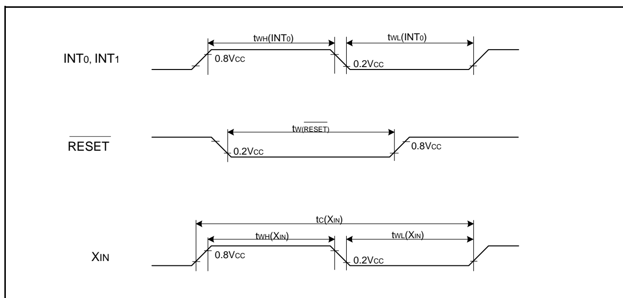
Fig 58. Timing chart
