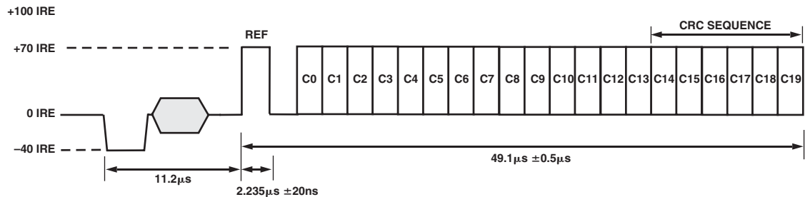
Figure 81. CGMS Waveform
