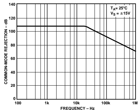
TPC 20. Common-Mode Rejection vs. Frequency @ \pm 15\text{V}
