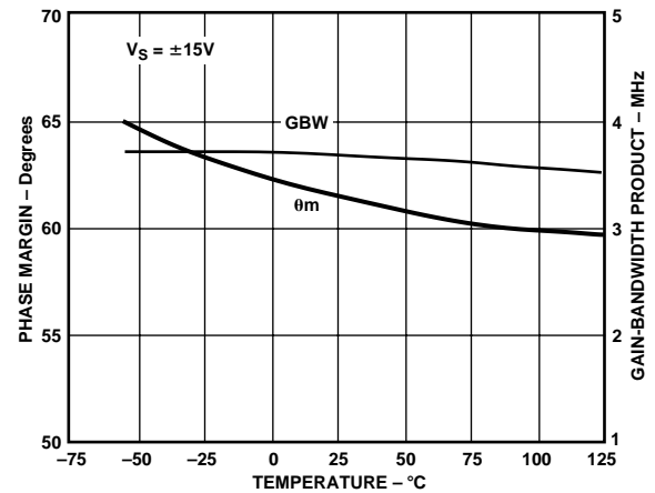
TPC 18. Gain Bandwidth Product and Phase Margin vs. Temperature @ \pm 15\text{V}
