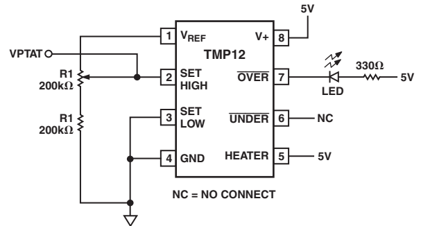
Figure 7. Measuring VPTAT with a Potentiometer
