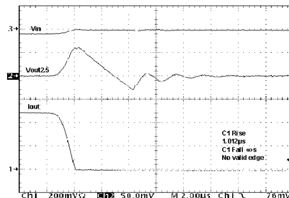
Figure 22 : Load Transient
