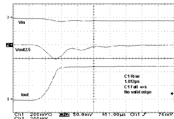
Figure 23 : Load Transient
