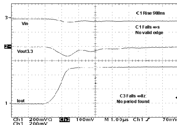
Figure 24 : Load Transient
