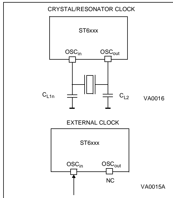
Figure 8. Oscillator Configurations
