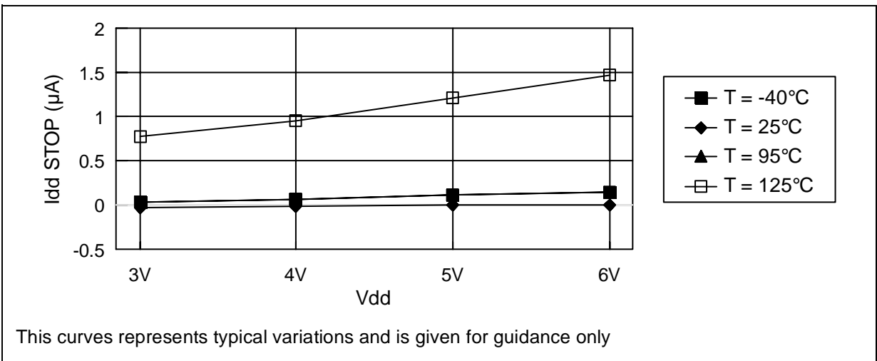
Figure 45. Idd STOP versus VDD for ROM devices
