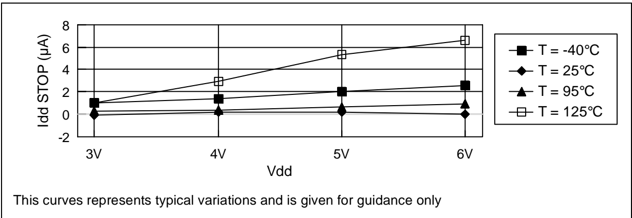
Figure 45. Idd STOP versus VDD for ROM devices
