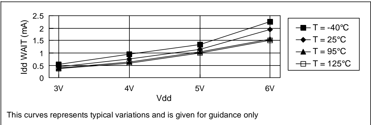
Figure 44. Idd STOP versus VDD for OTP devices
