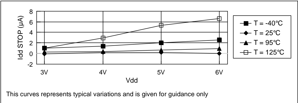
Figure 44. Idd STOP versus VDD for ROM devices
