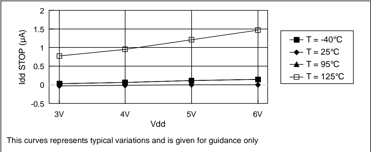
Figure 44. Idd STOP versus VDD for ROM devices
