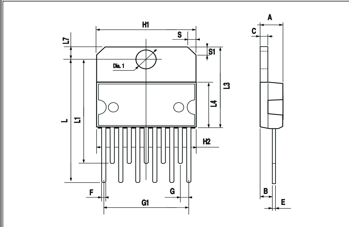
Multiwatt11 (In-Line)
