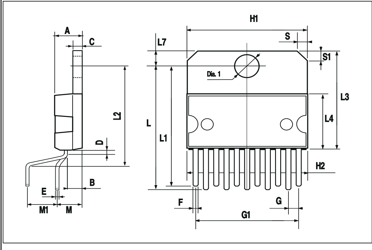
Multiwatt11 V
