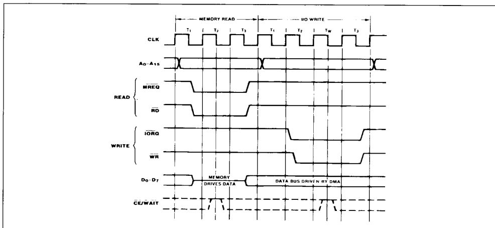
Figure 12 : Memory-to-I/O Transfer.
