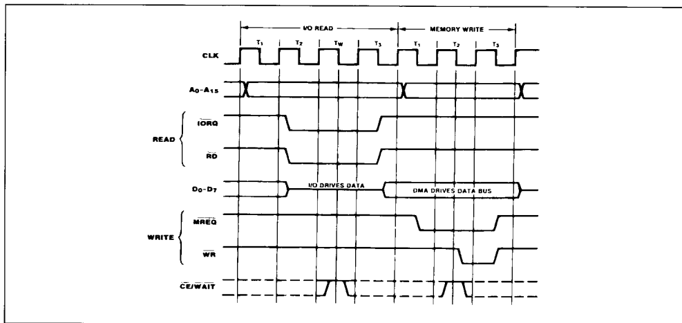
Figure 13 : I/O-to-Memory Transfer.
