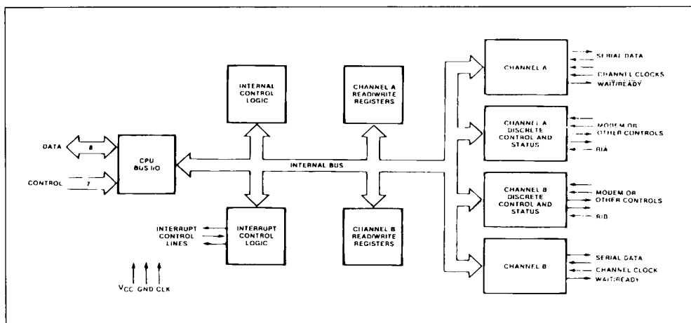
Figure 3 : Block Diagram.
