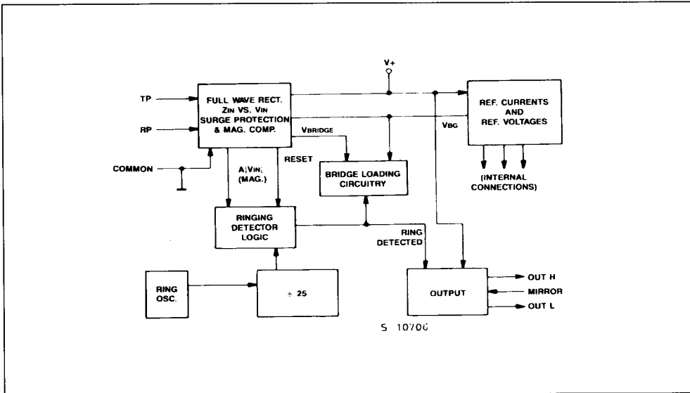
Figure 1 : Functional Diagram.
