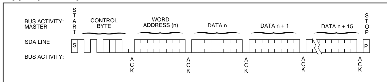
FIGURE 8-1: PAGE WRITE
