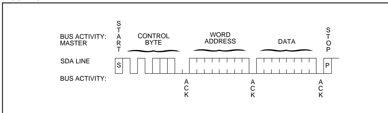
FIGURE 5-1: BYTE WRITE
