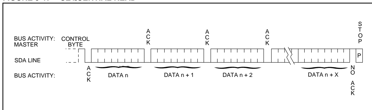
FIGURE 9-1: SEQUENTIAL READ
