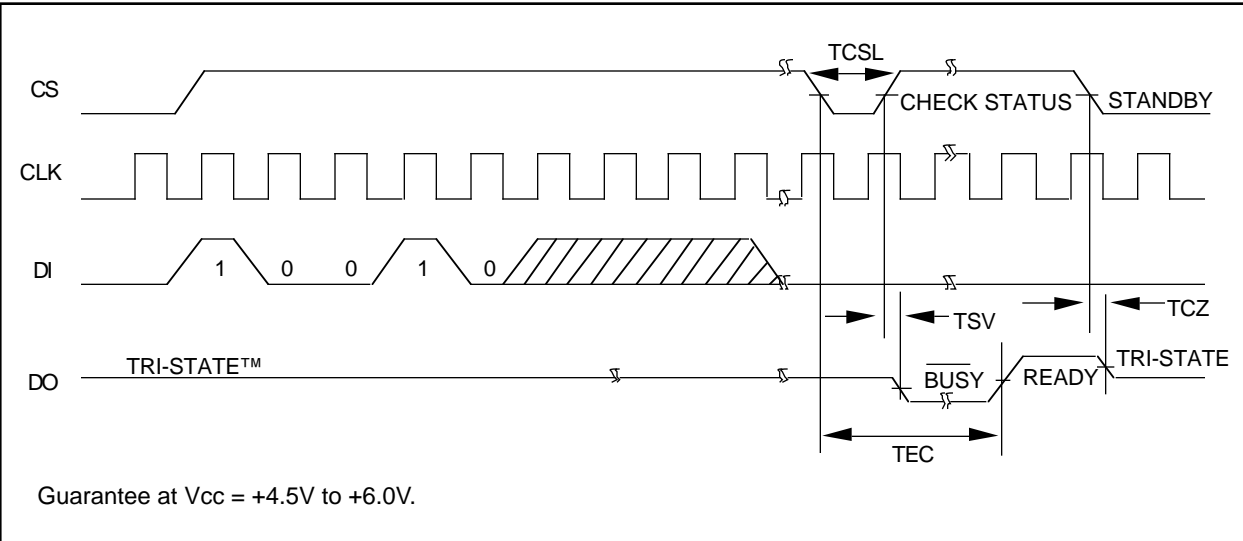
FIGURE 9-8: ERASE TIMING
