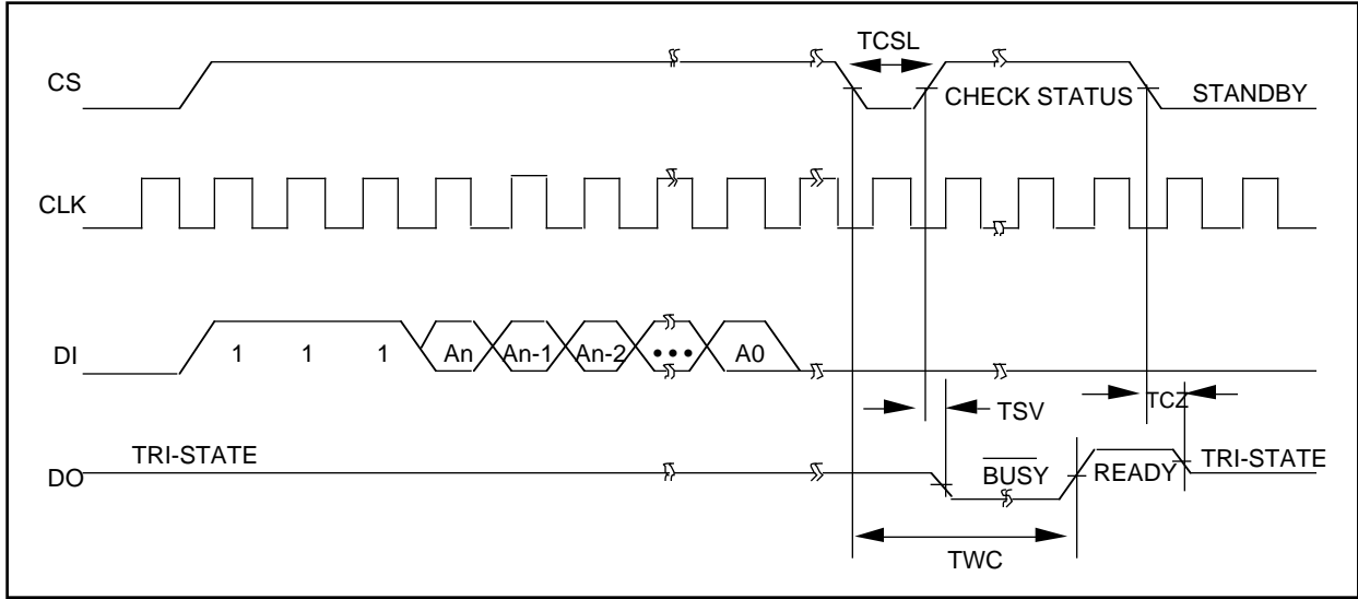
FIGURE 9-8: ERASE TIMING
