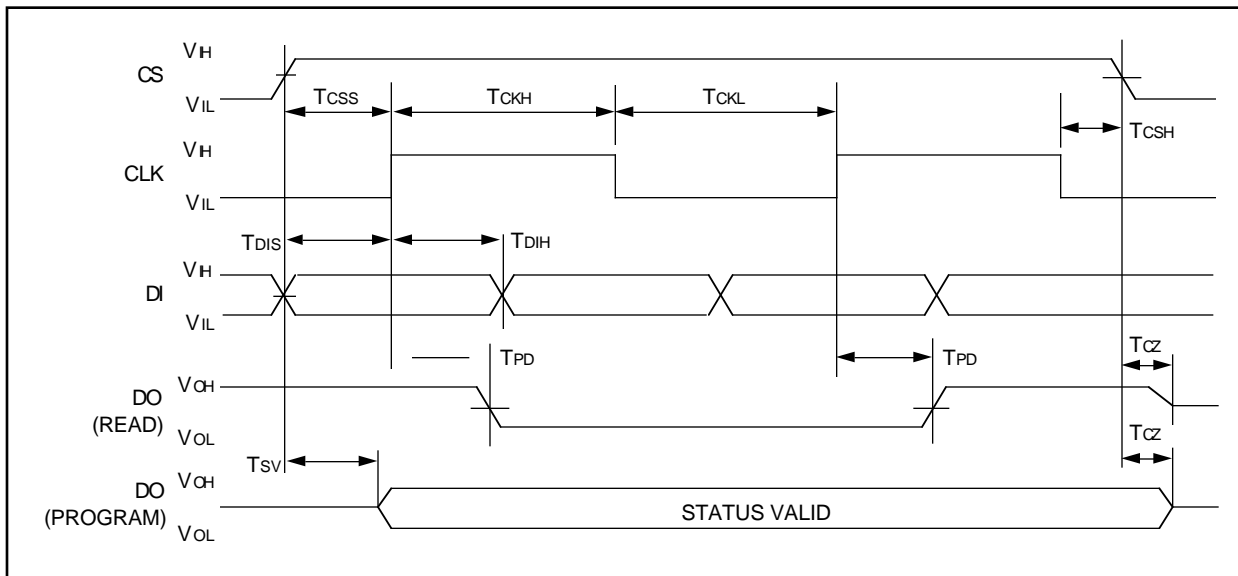
FIGURE 9-2: READ TIMING
