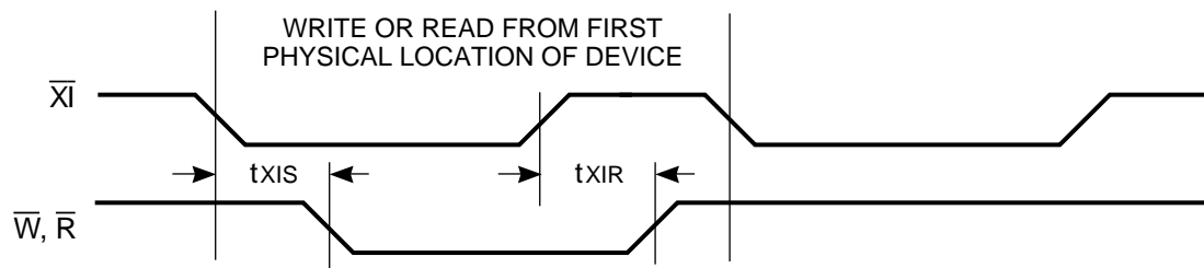
FIGURE 13. EXPANSION-IN TIMING
