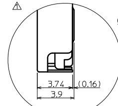
DETAIL B (5:1)
