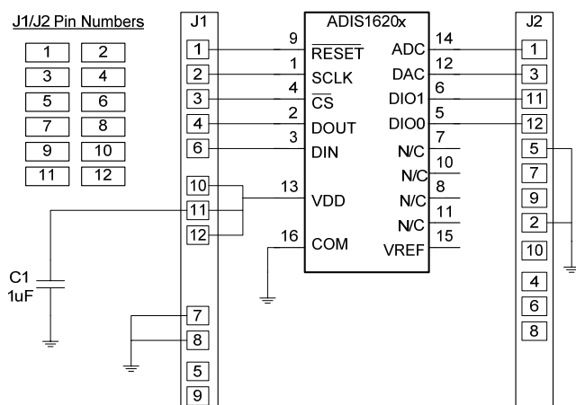
Figure 1. ADIS1620x/PCB Schematic
