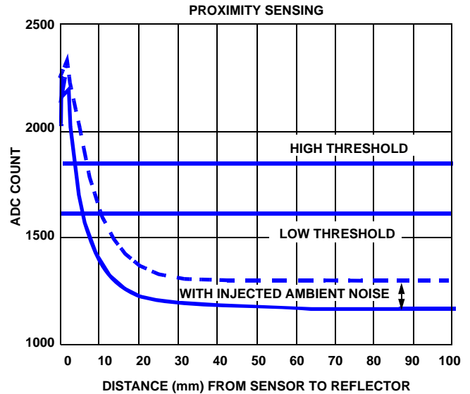
FIGURE 21. PROXIMITY RESPONSE CURVE vs DISTANCE FOR HUMAN SKIN
