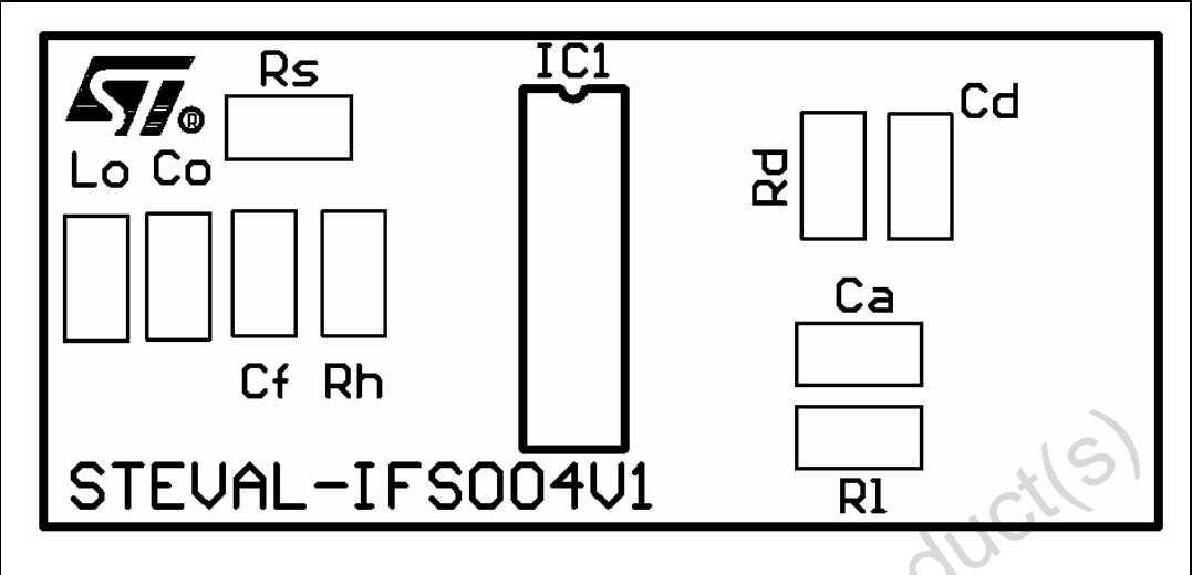
Figure 3. Bottom overlay (1)
