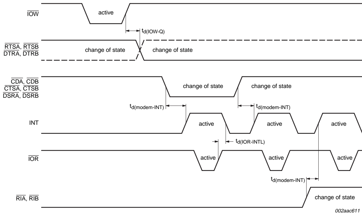
Fig 14. Modem input/output timing in 16 mode
