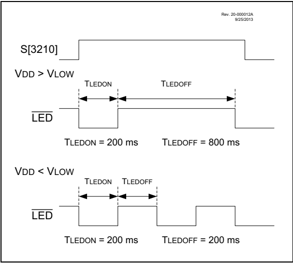
FIGURE 7-1: LED OPERATION
