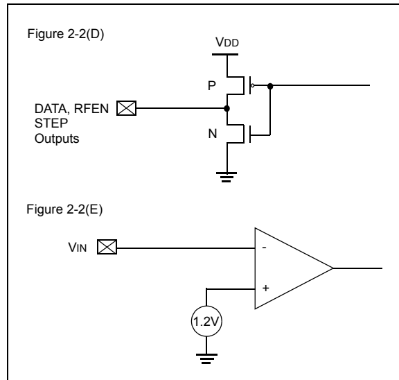
FIGURE 2-2: I/O CIRCUITS
