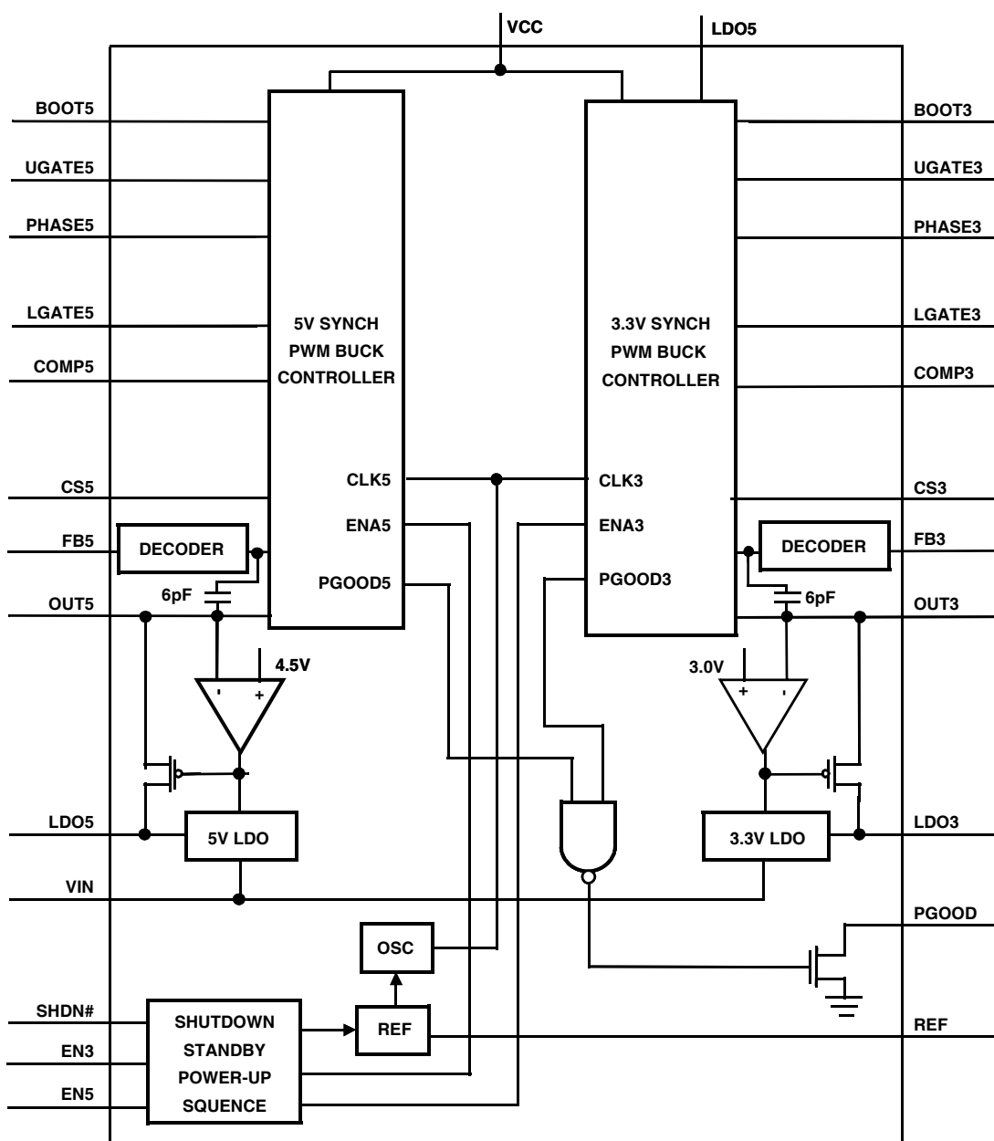
FIGURE 30. FUNCTIONAL DIAGRAM
