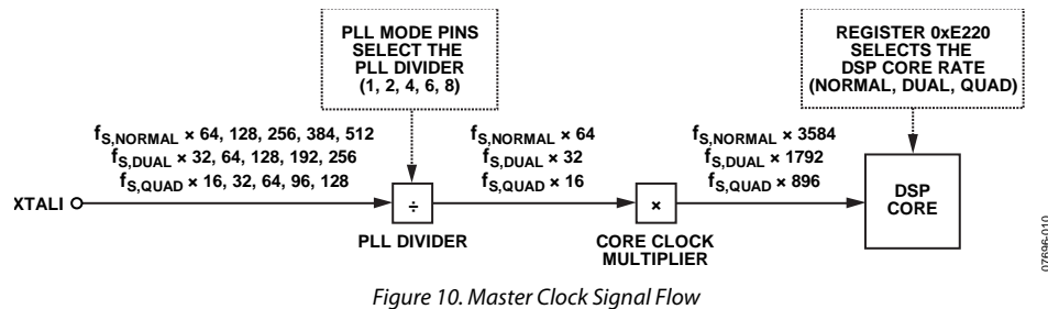
Figure 10. Master Clock Signal Flow
