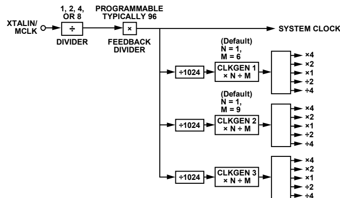
Figure 17. PLL and Clock Generators Block Diagram
