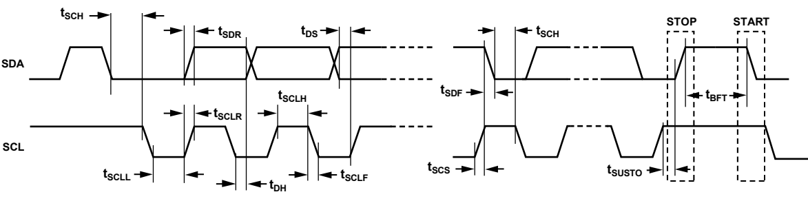
Figure 6. I 2 C Slave Port Timing Specifications
