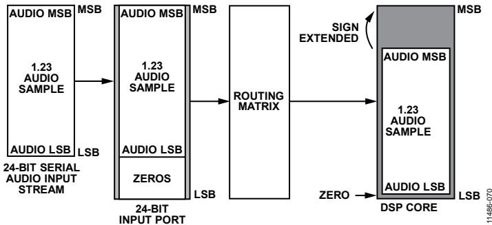
Figure 67. 24-Bit Serial Input Example
