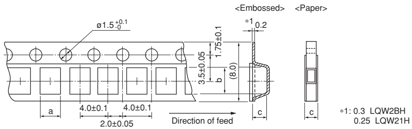
Dimension of the cavity of embossed tape is measured at the bottom side.
