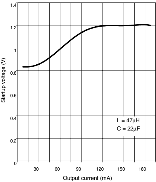
Figure 5. Startup Voltage vs Output Current
