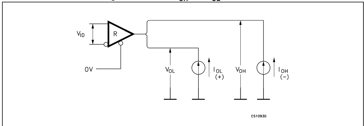
Figure 5. Receiver V_{OH} and V_{OL} test circuit
