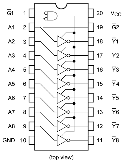
74VHC540FT
