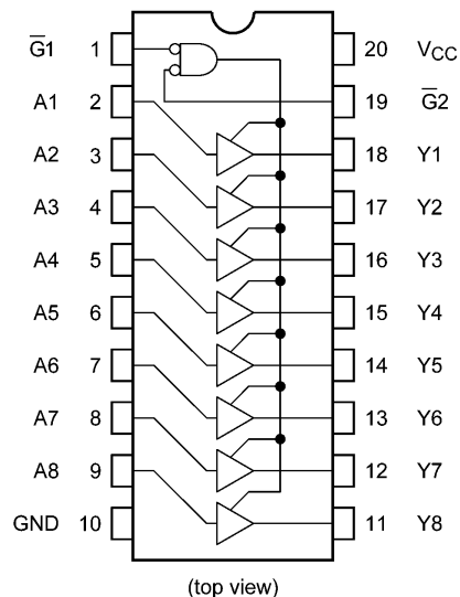
74VHC541FT
