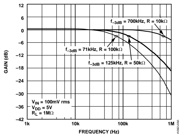
Figure 30. -3 dB Bandwidths
