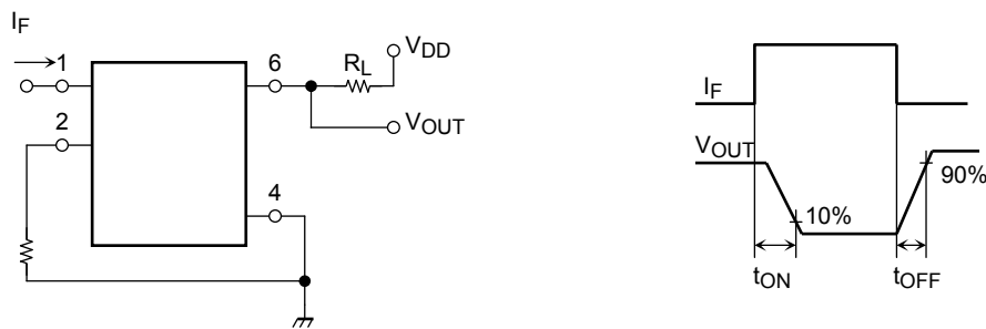
Note 2: Switching time test circuit
