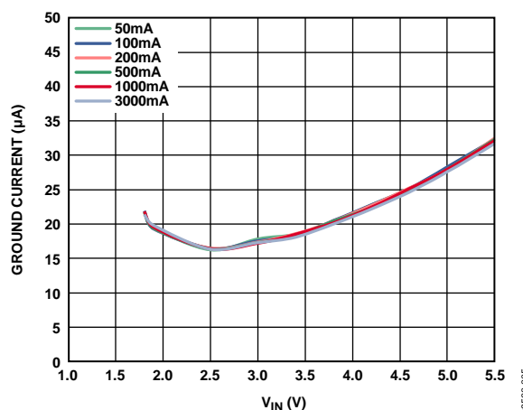
Figure 5. Ground Current vs. Input Voltage ( V_{IN} )
