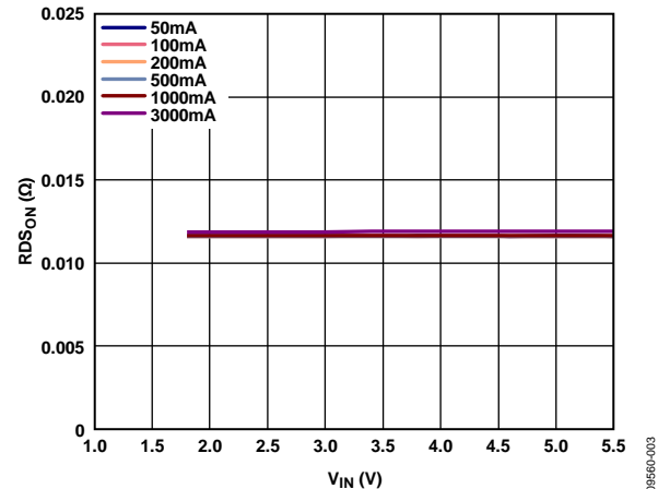
Figure 3. R_{DS_{ON}} vs. Input Voltage ( V_{IN} ) Different Load Currents
