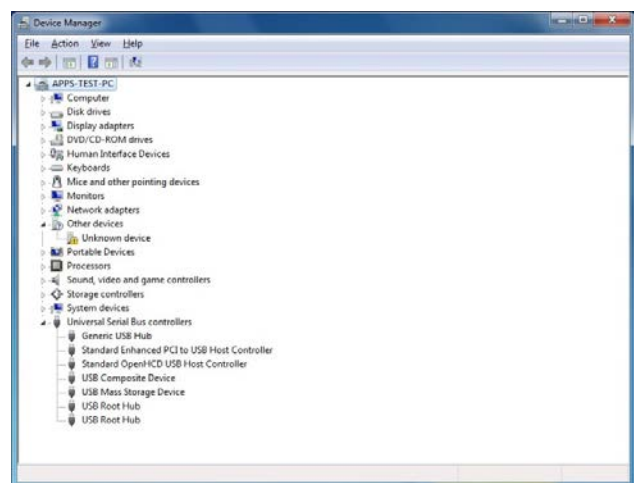
Figure 5. Device Manager
