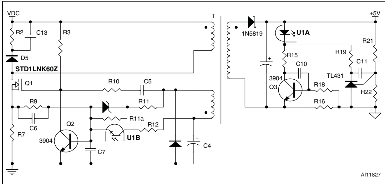
Figure 1. RCC control circuit components schematic
