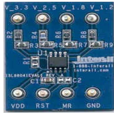
FIGURE 11. ISL88041EVAL1 PHOTO
