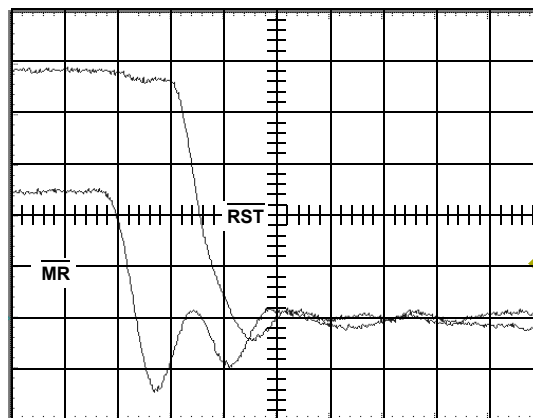
MR = 1V/DIV RST = 1V/DIV 10ns/DIV
