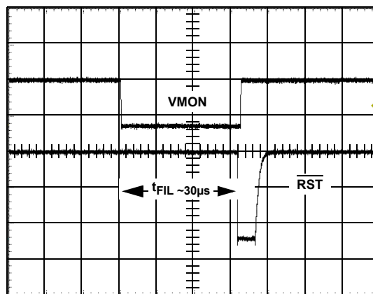
RST = 2V/DIV VMON = 1V/DIV 10μs/DIV
