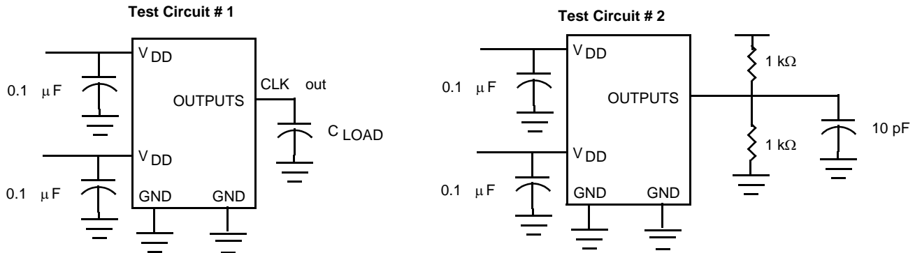
For parameter t_8 (output slew rate) on -1H devices
