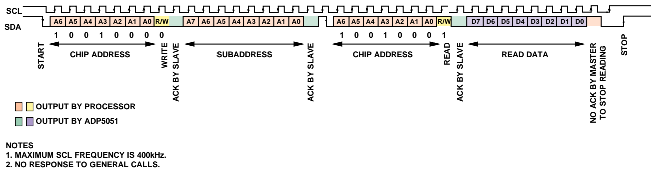
Figure 58. I 2 C Read from Register
