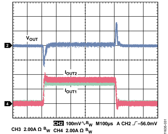
Figure 28. Load Transient, Channel 1/Channel 2 Parallel Output, 0 A to 6 A, V_{IN} = 12\text{ V} , V_{OUT} = 3.3\text{ V} , f_{SW} = 600\text{ kHz} , L = 4.7\text{ }\mu\text{H} , C_{OUT} = 47\text{ }\mu\text{F} \times 4
