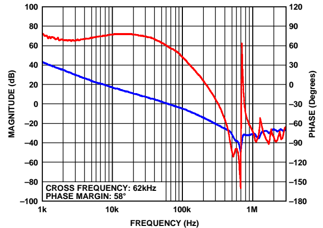
Figure 60. Bode Plot for 1.2 V Output
