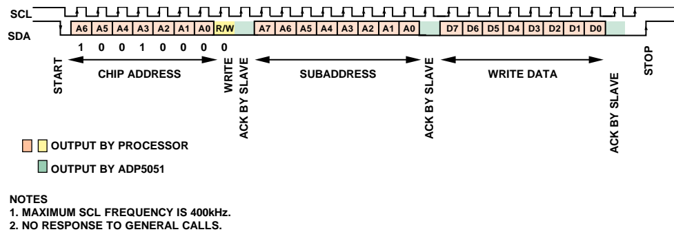
Figure 57. I 2 C Write to Register
