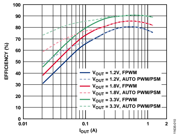
Figure 12. Channel 3/Channel 4 Efficiency Curve, V_{IN} = 12\text{ V} , f_{SW} = 600\text{ kHz} , FPWM and and Automatic PWM/PSM Modes
