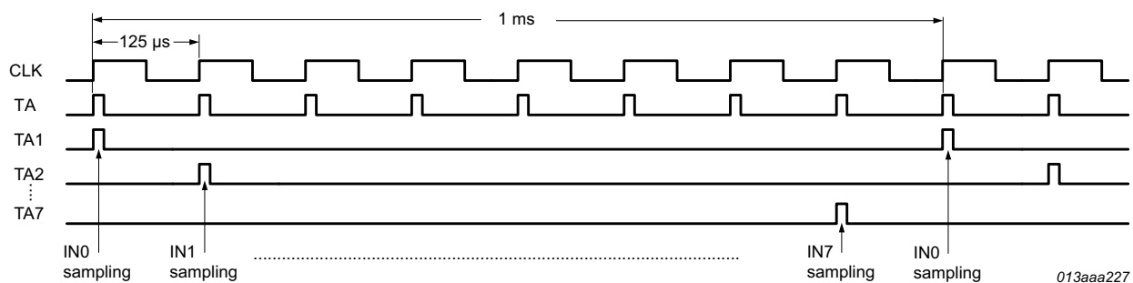
Fig 3. Timing diagram of sensor sampling
