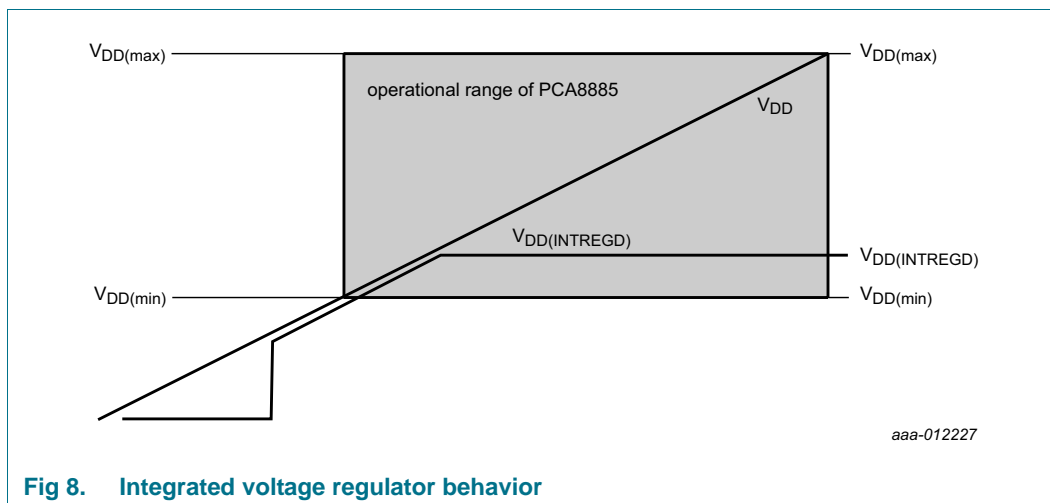
Figure 8 illustrates the behavior of the integrated voltage regulator. The gray area covers the operational range of the PCA8885. The analog part of the circuit and the switch logic is powered from V_{DD(INTREGD)} . The I 2 C interface and the registers are powered from V_{DD} . Therefore the I 2 C interface remains accessible in sleep mode, and the register values are maintained when V_{DD(INTREGD)} is powered off.
