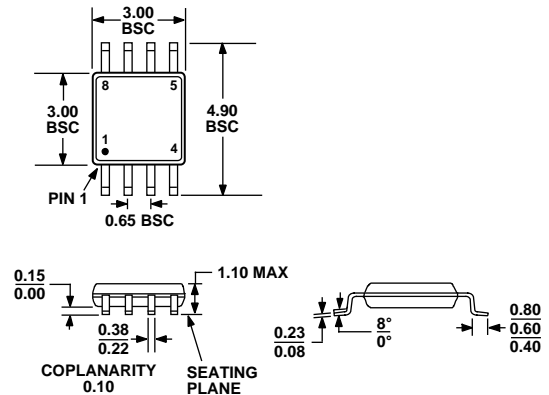
Figure 41. 8-Lead Mini Small Outline Package (MSOP)
