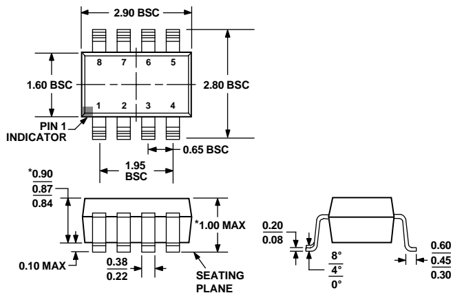
Figure 40. 8-Lead Thin Small Outline Transistor Package (TSOT)
