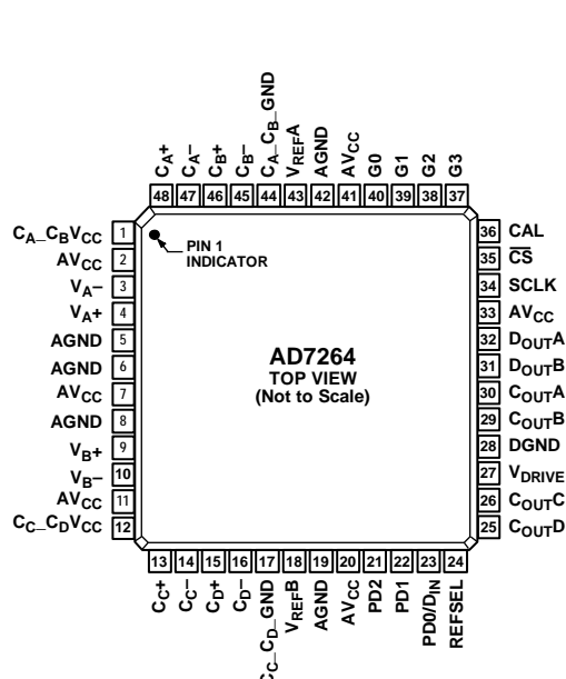
Figure 3. 48-Lead LQFP Pin Configuration
