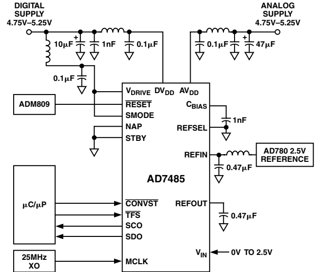
Figure 11. Typical Connection Diagram
