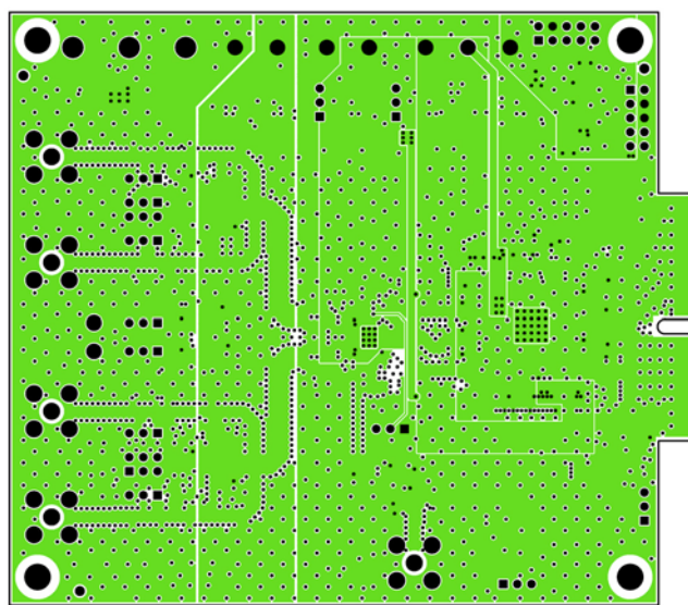
Figure 3. Layer 3, Power Plane
