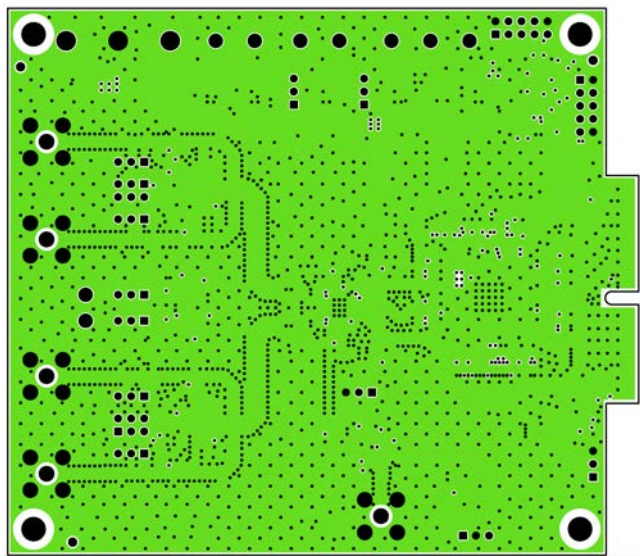
Figure 2. Layer 2, Ground Plane
