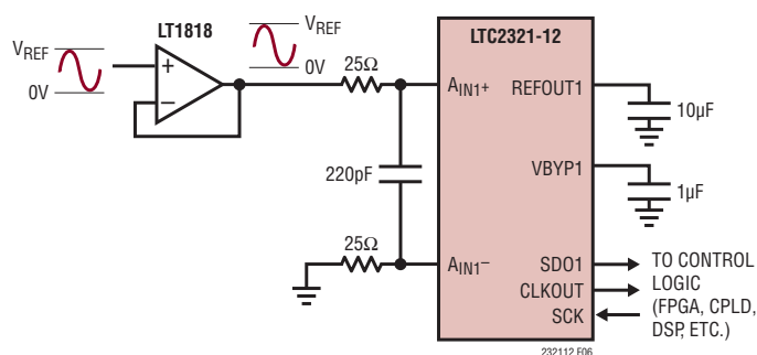
Figure 6. Pseudo-Differential Unipolar Application Circuit
