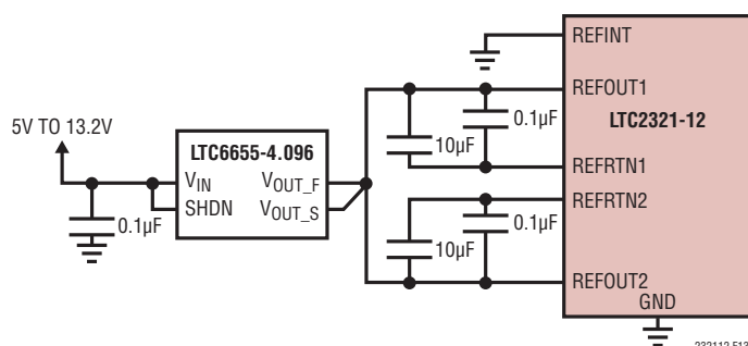
(13b) LTC2321-12 with a Shared External Reference Circuit
