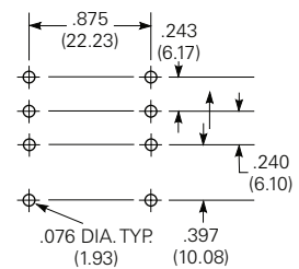
2 pole version
