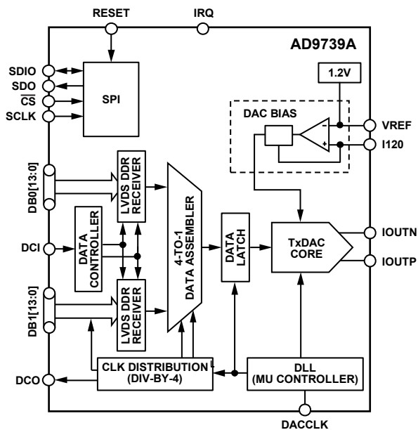
Figure 74. Functional Block Diagram of the AD9739A
