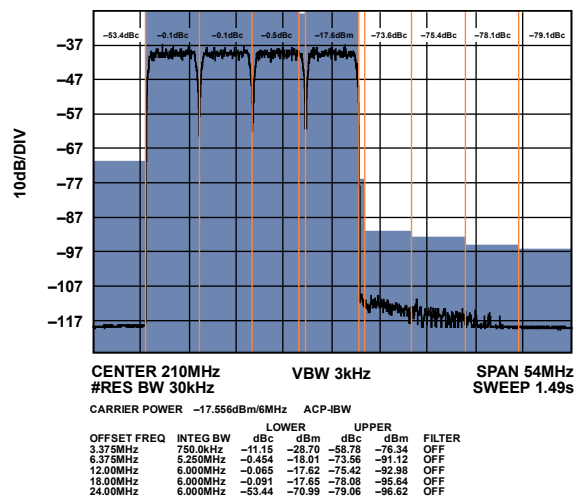
Figure 43. Low Band Narrow-Band ACLR (Worst Side)
