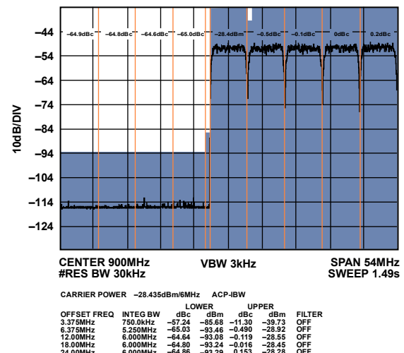
Figure 57. High Band Narrow-Band ACLR (Worst Side)
