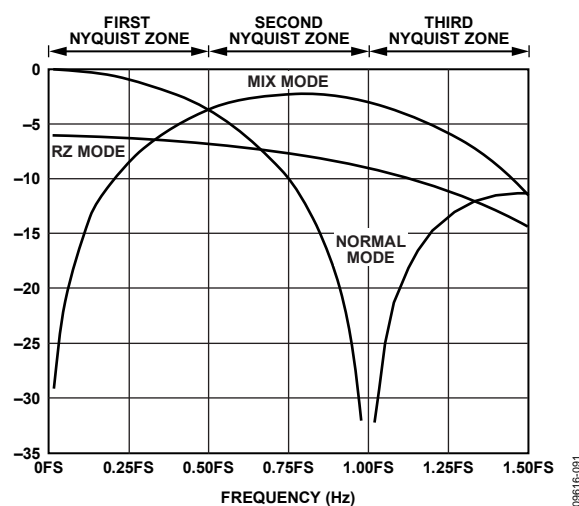
Figure 88. Sinc Roll-Off for Each Analog Operating Mode
