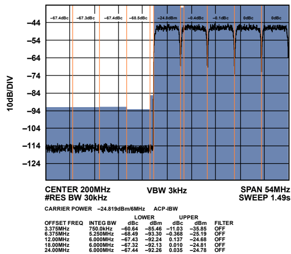
Figure 55. Low Band Narrow-Band ACLR (Worst Side)
