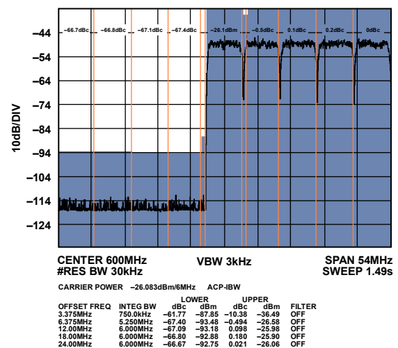
Figure 56. Mid Band Narrow-Band ACLR (Worst Side)
