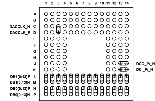
Figure 4. Digital LVDS Clock Supply Pins (Top View)
