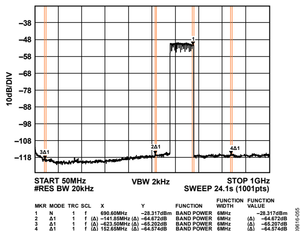
Figure 53. Mid Band Wideband ACLR
