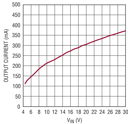
Figure 1. V_{OUT1} Typical Maximum Output Current vs V_{IN} When V_{OUT2} is not Loaded
