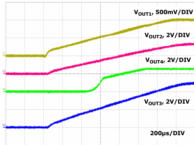
FIGURE 11. SOFT-START CURVES
