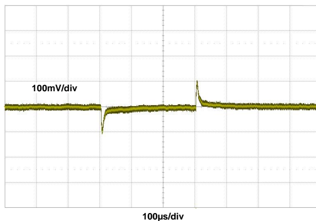
FIGURE 12. 1V OUT TRANSIENT RESPONSE, I OUT = 0A to 20A, FSW=350kHz, LOAD CURRENT SLEW RATE: 10A/µs
