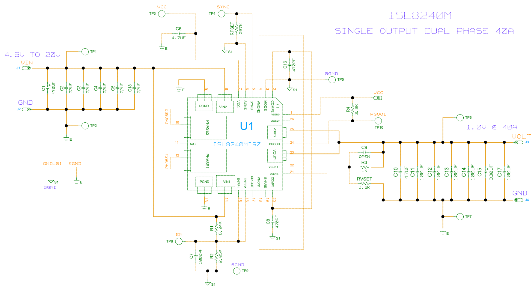
FIGURE 2. ISL8240MEVAL3Z BOARD SCHEMATIC
