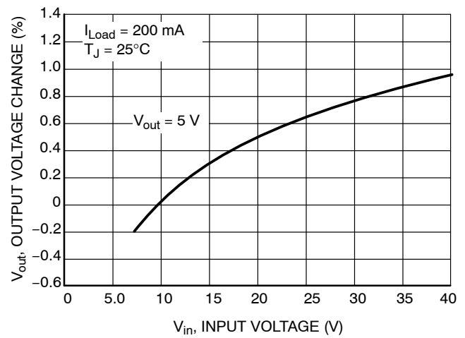
Figure 4. Line Regulation
