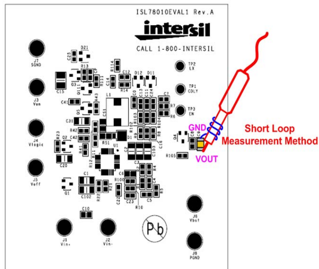
FIGURE 5. OUTPUT RIPPLE/NOISE MEASUREMENT
