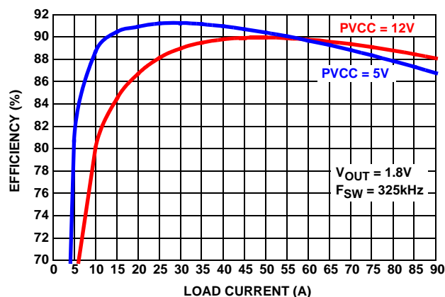
FIGURE 15. EFFICIENCY vs LOAD CURRENT
