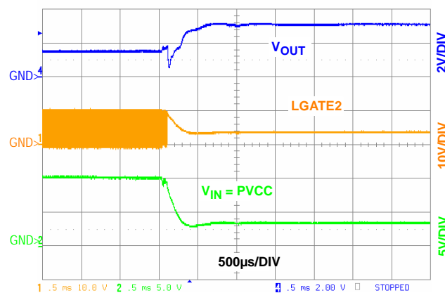
FIGURE 13. ISL6308AEVAL1Z PRE-POR OVERVOLTAGE PROTECTION
